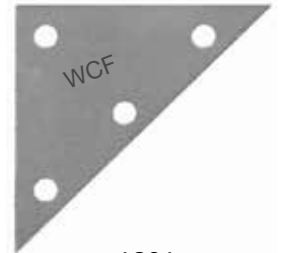
•1801 Triangular Hanging Plate L69 x 69 x T1.0mm Zinc Plated
